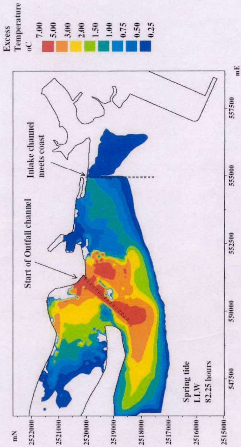
Figure 6.1.5: Modelled temperature distribution during peak lowest low water tide (Spring)
