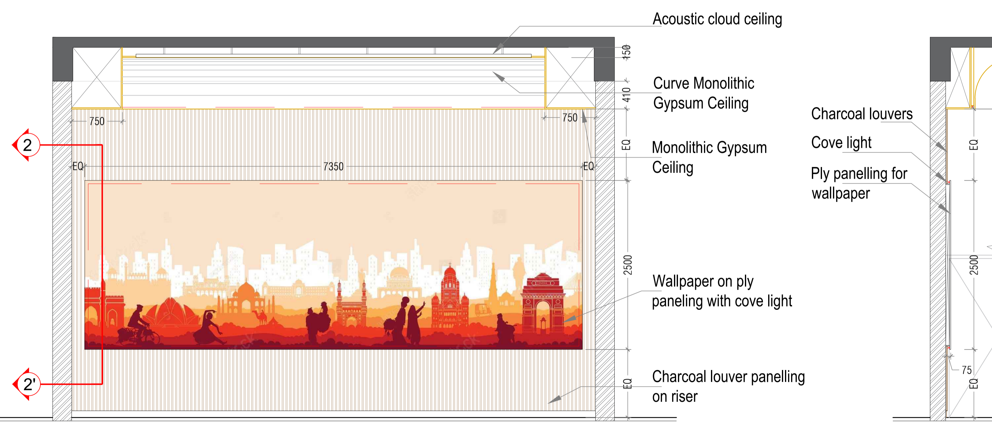
SECTION AT DD
